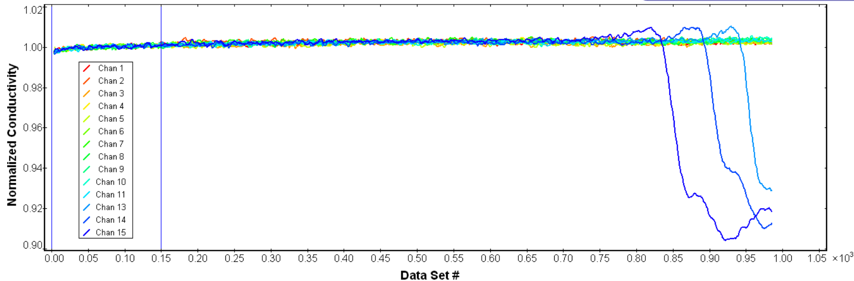
Conductivity vs. Set - 630.9 kHz - (Moving average, n = 5)
