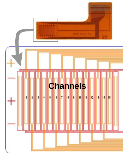
MWM-Array FA116
