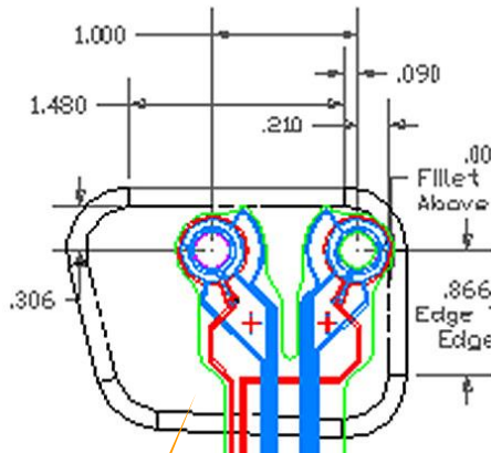
MWM-Array FA138
