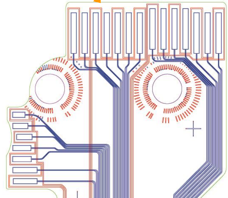
MWM-Array FA140
