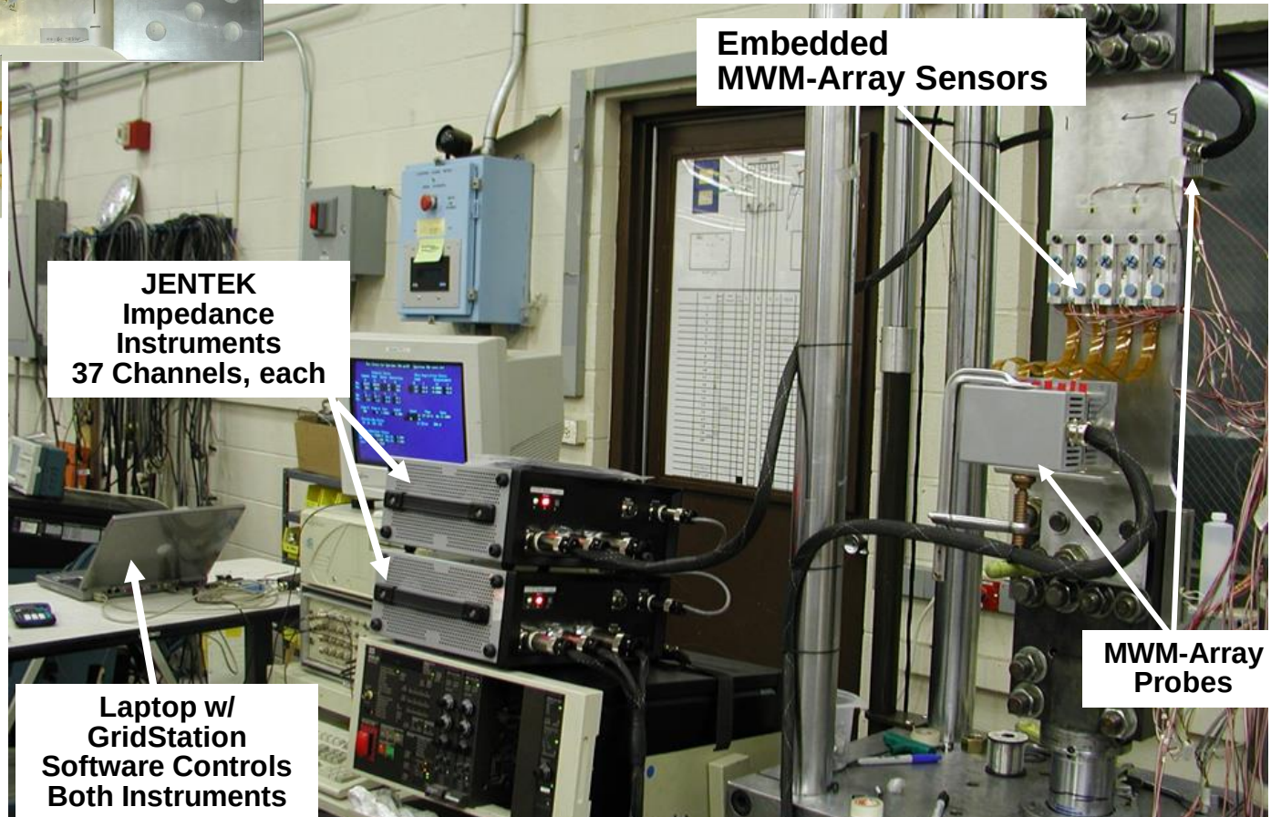
10-Hole Specimen with MWM-Array Networks
