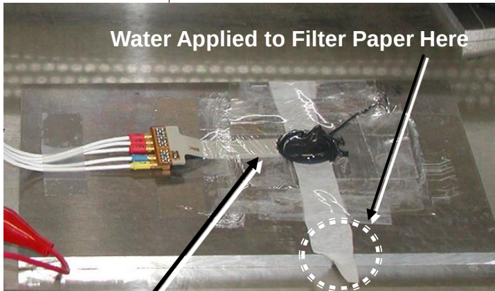
IDED (DS04) sensor
